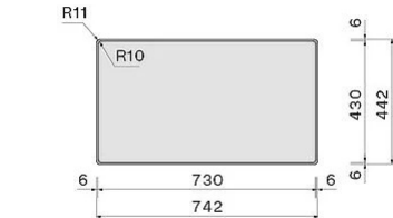
Cut-out size / Flushmount
